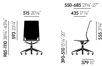
Meda Chair, zonder armleuningen
